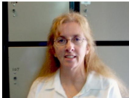
Association Manager
